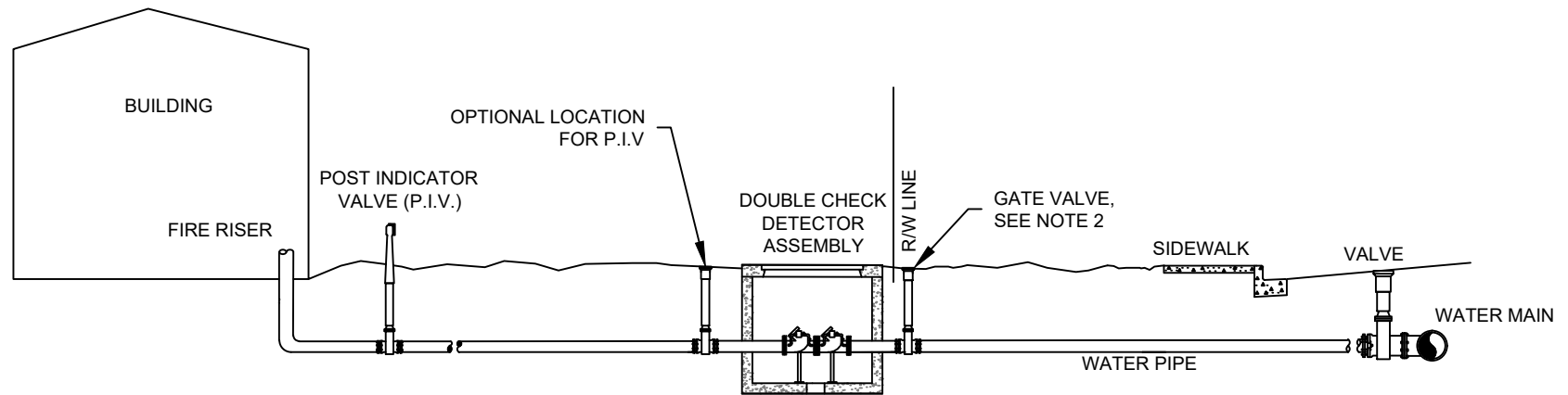
FIRE SPRINKLER SYSTEM LINE
