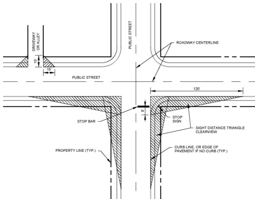
Figure 8.1 Sight Distance Triangle Clearview
