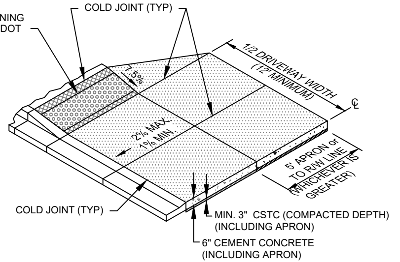
COMMERCIAL APPROACH - TYPE 2
