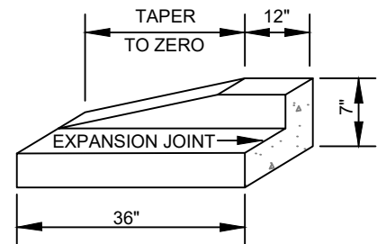
CURB TERMINAL END
