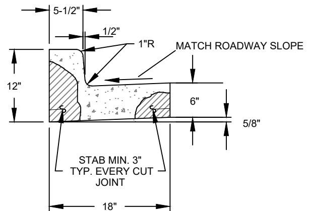
TYPE "A" BARRIER CURB AND GUTTER
