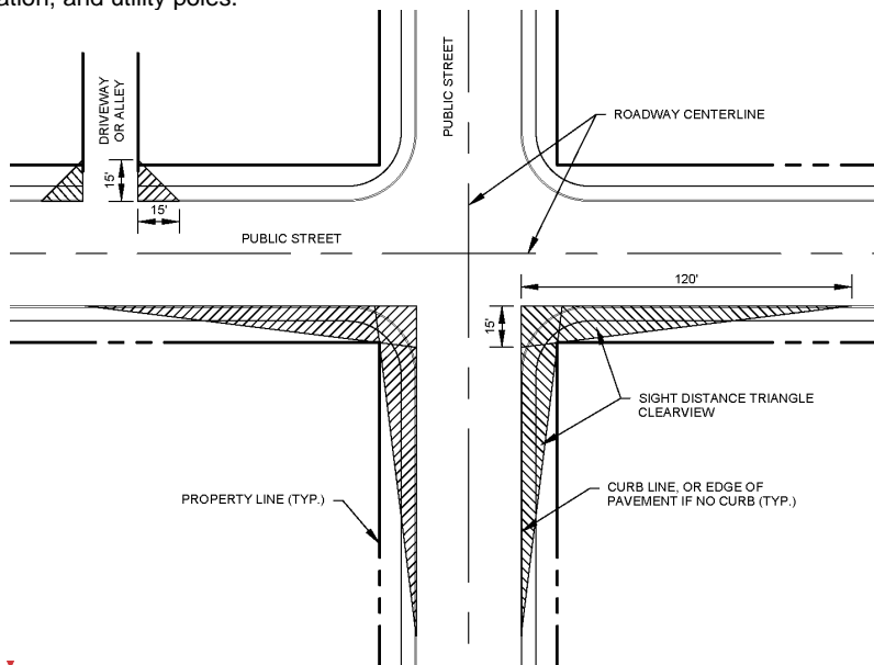
Figure 8.1 Sight Distance Triangle Clearview
