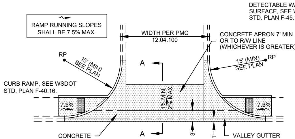
COMMERCIAL APPROACH - TYPE 1
